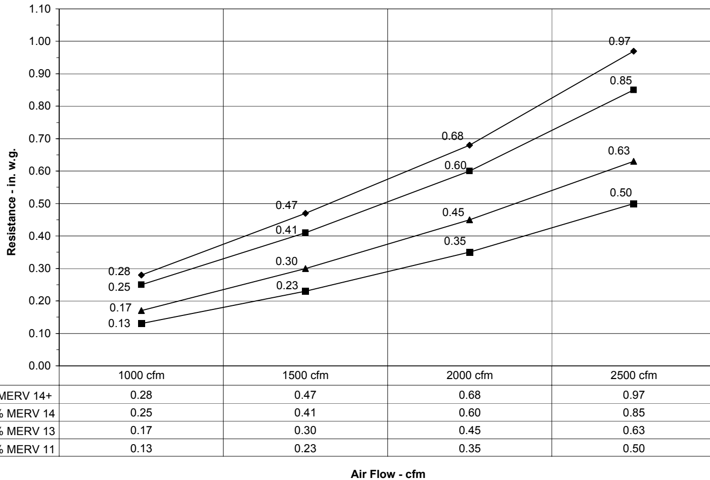
Resistance vs. Air Flow - Clean Device
